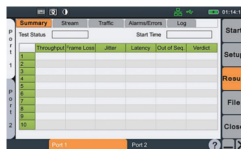
Ethernet traffic generation measurement screen
