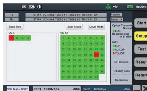
SDH insert / discard specified tributary measurement screen
