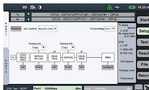
OTN BERT measurement screen
